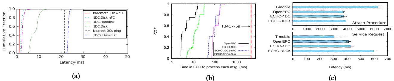
Figure 11: Latency vs. reliability trade-off: (a) Network latency CDF for ZooKeeper write. Baremetal showed optimal, non-virtualized performance; (b) CDF of message latency for an Attach Request procedure with different deployments and different ZK configurations; (c) UE-perceived latency for Attach Request procedure (top) and Service Request procedure (bottom), compared with T-mobile
